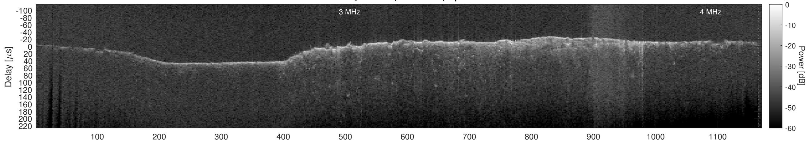
Orbit 10969, Cluttergram
