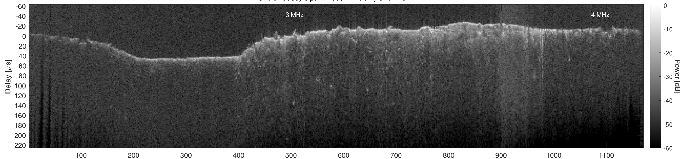
Orbit 10969, Cluttergram
