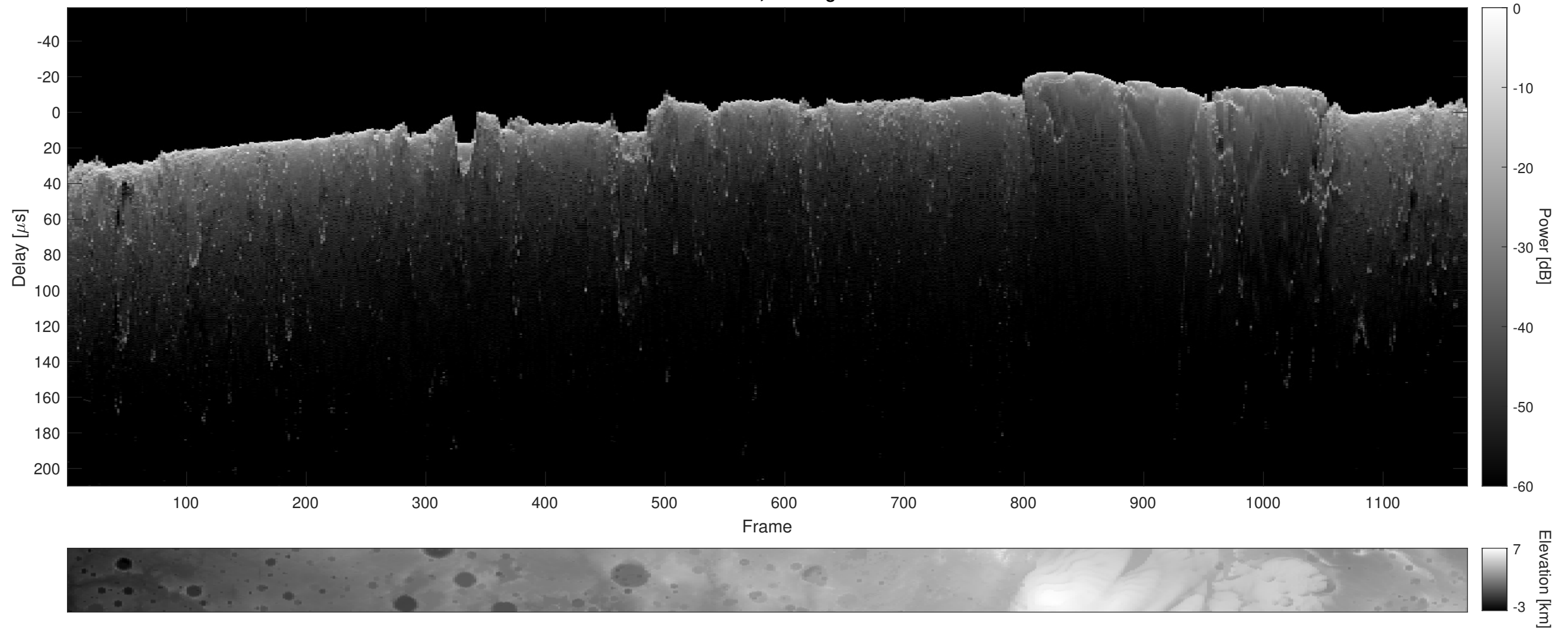
Orbit 10970, Cluttergram
