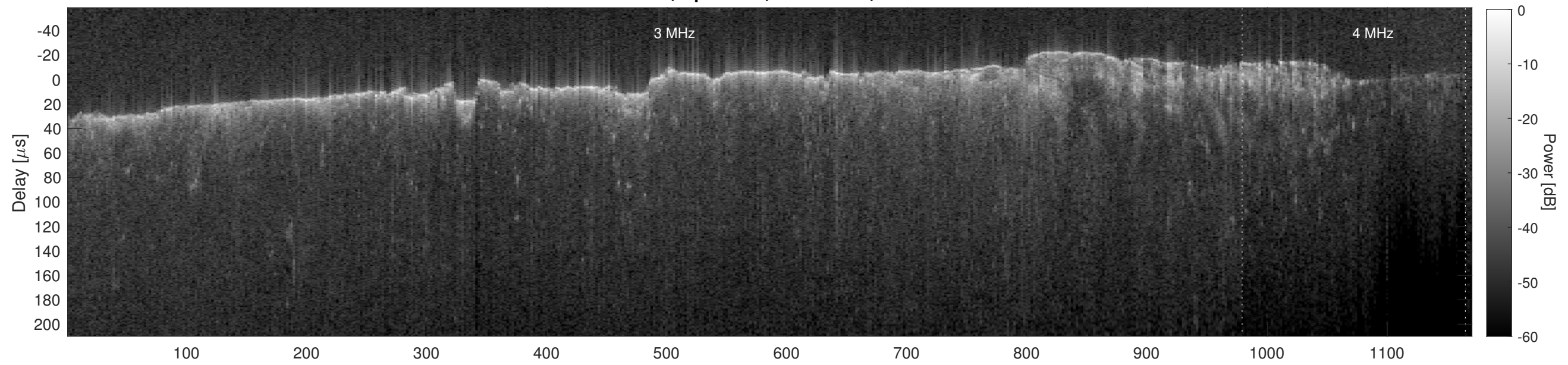
Orbit 10970, Cluttergram
