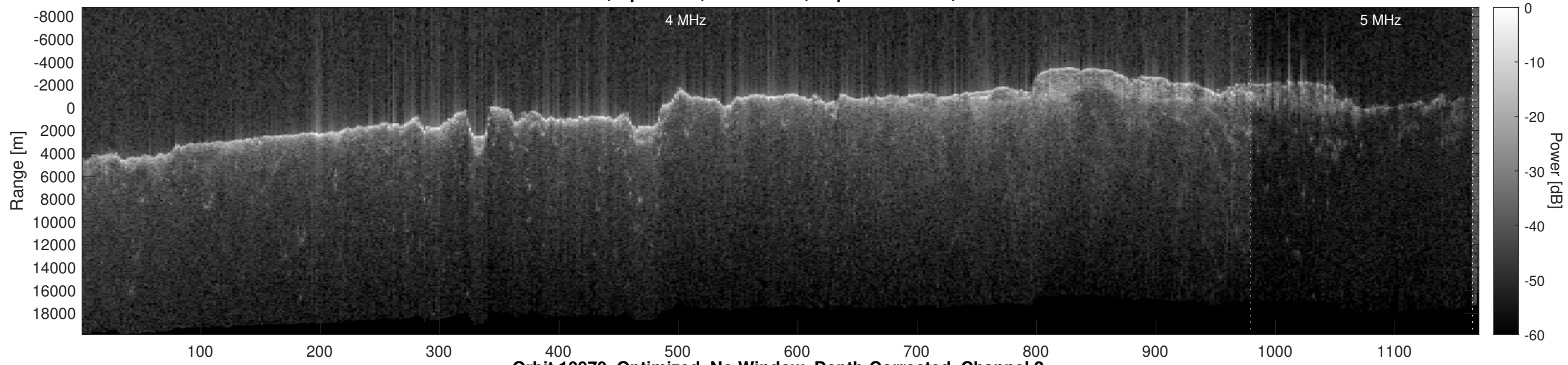
Orbit 10970, Optimized, No Window, Depth-Corrected, Channel 2
