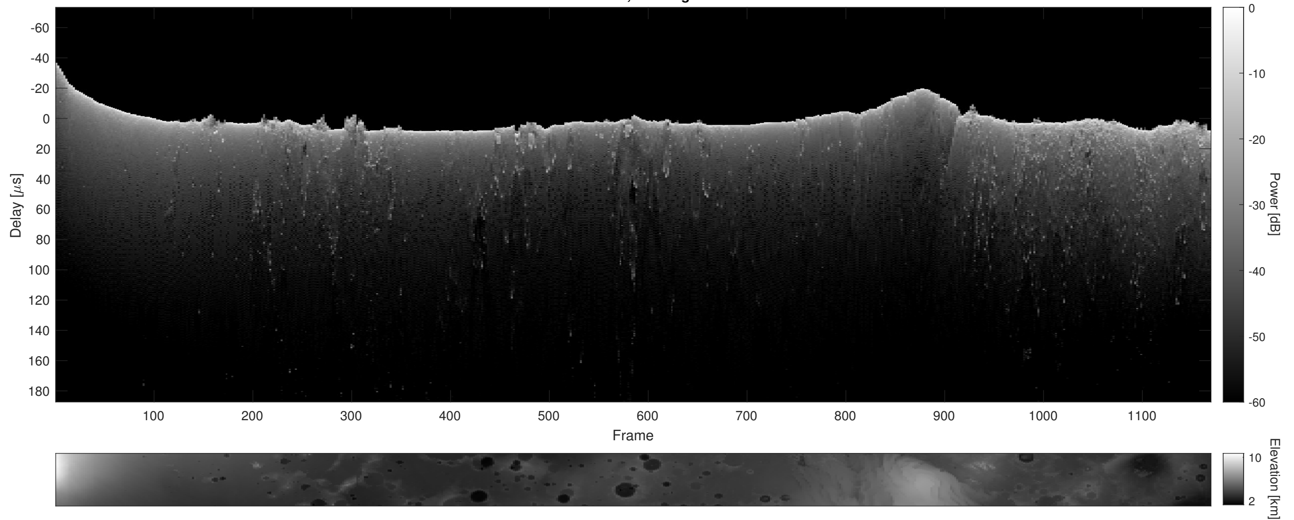
Orbit 10971, Cluttergram
