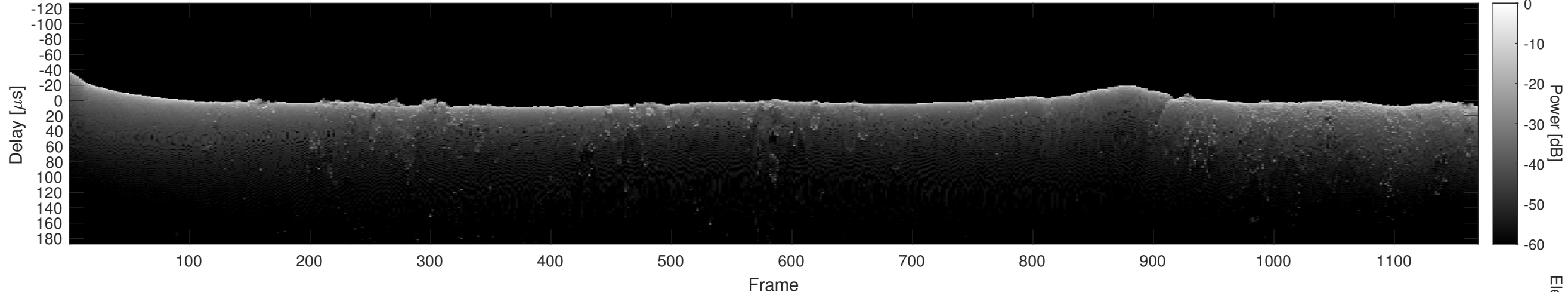
Orbit 10971, Cluttergram
