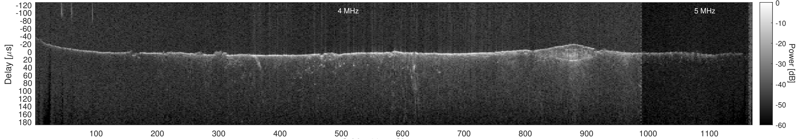
Orbit 10971, Cluttergram
