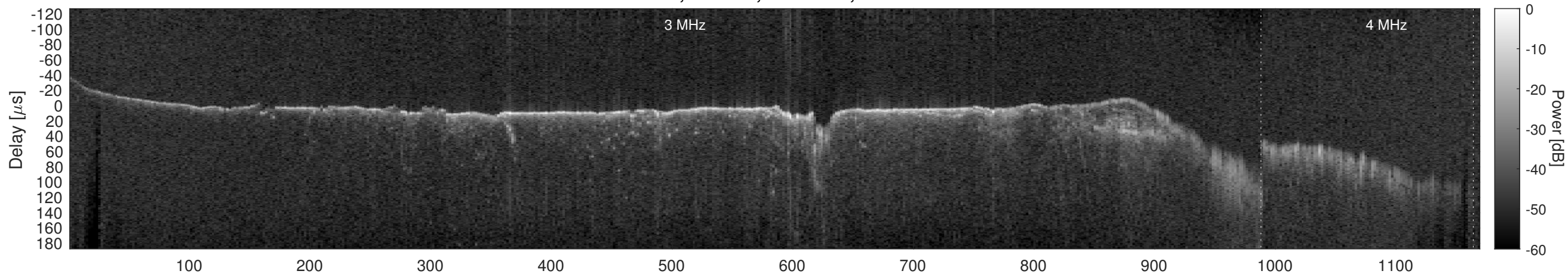
Orbit 10971, Window, Channel 2, Chapman
