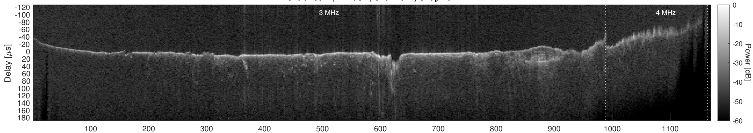
Orbit 10971, Window, Channel 2, Optimized
