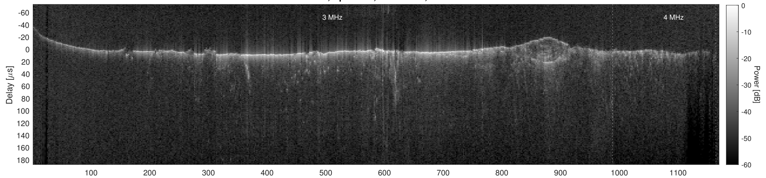
Orbit 10971, Cluttergram
