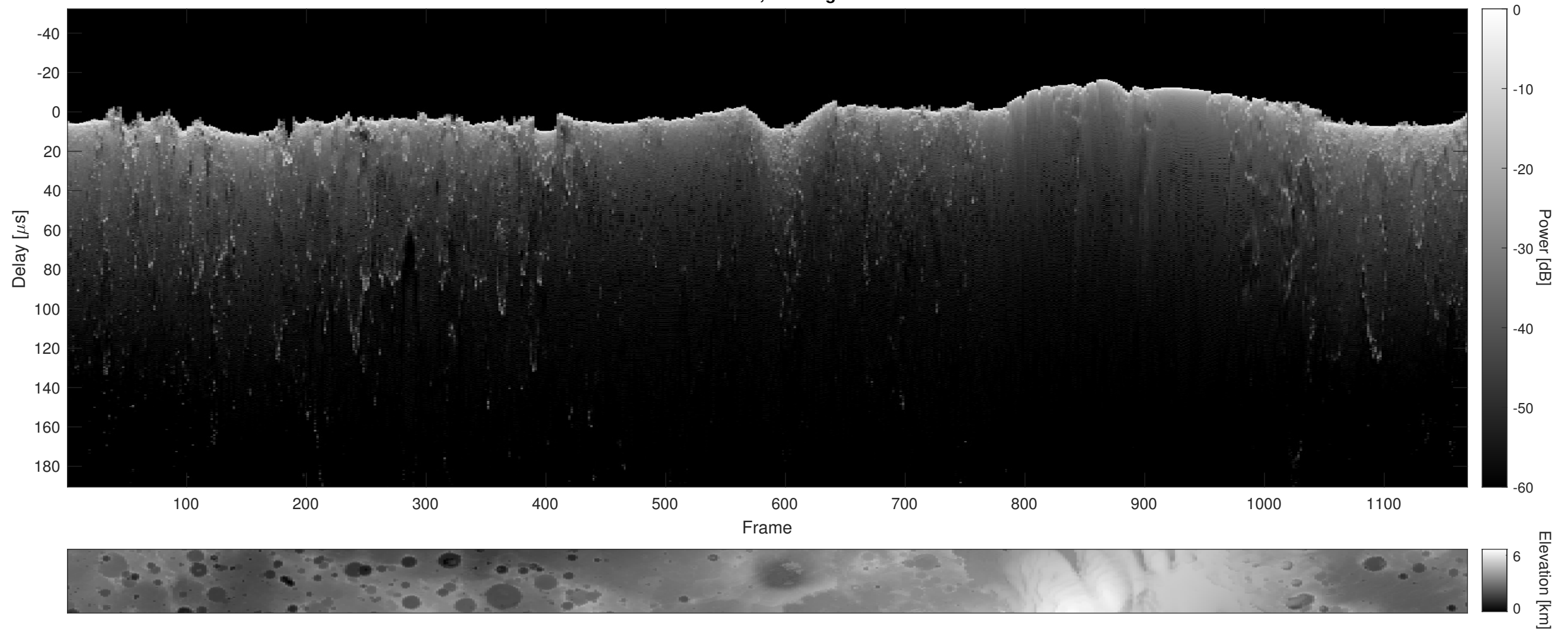
Orbit 10973, Cluttergram
