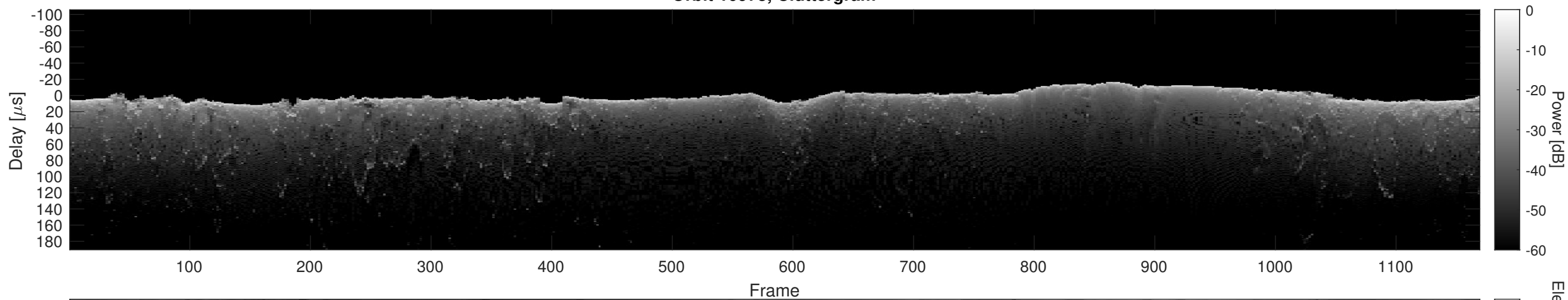
Orbit 10973, Cluttergram
