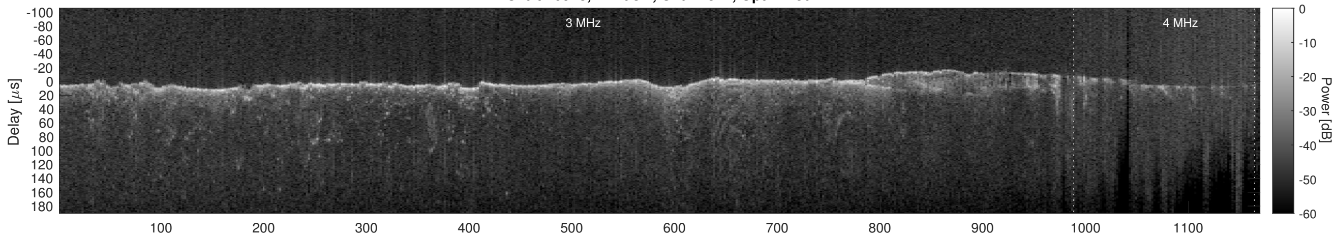
Orbit 10973, Cluttergram
