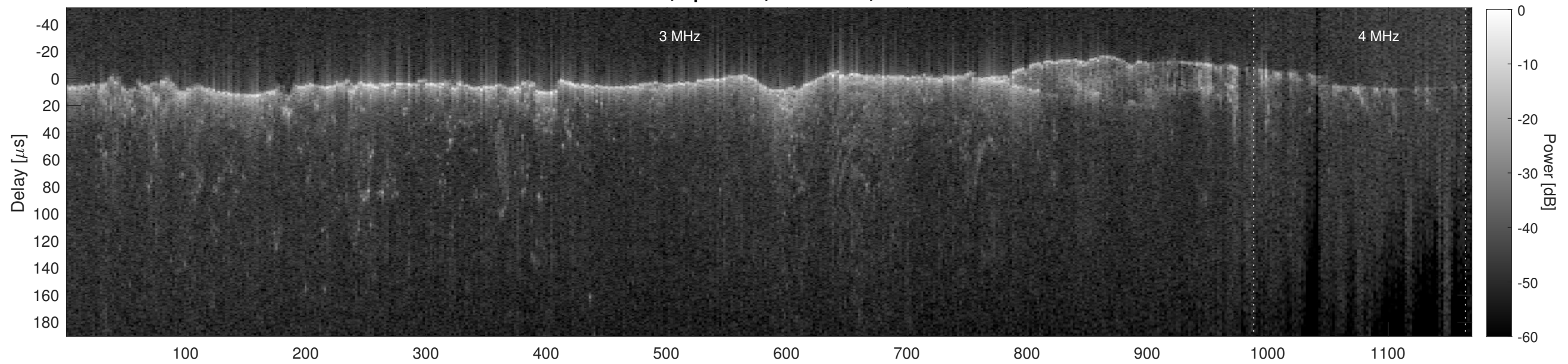
Orbit 10973, Cluttergram
