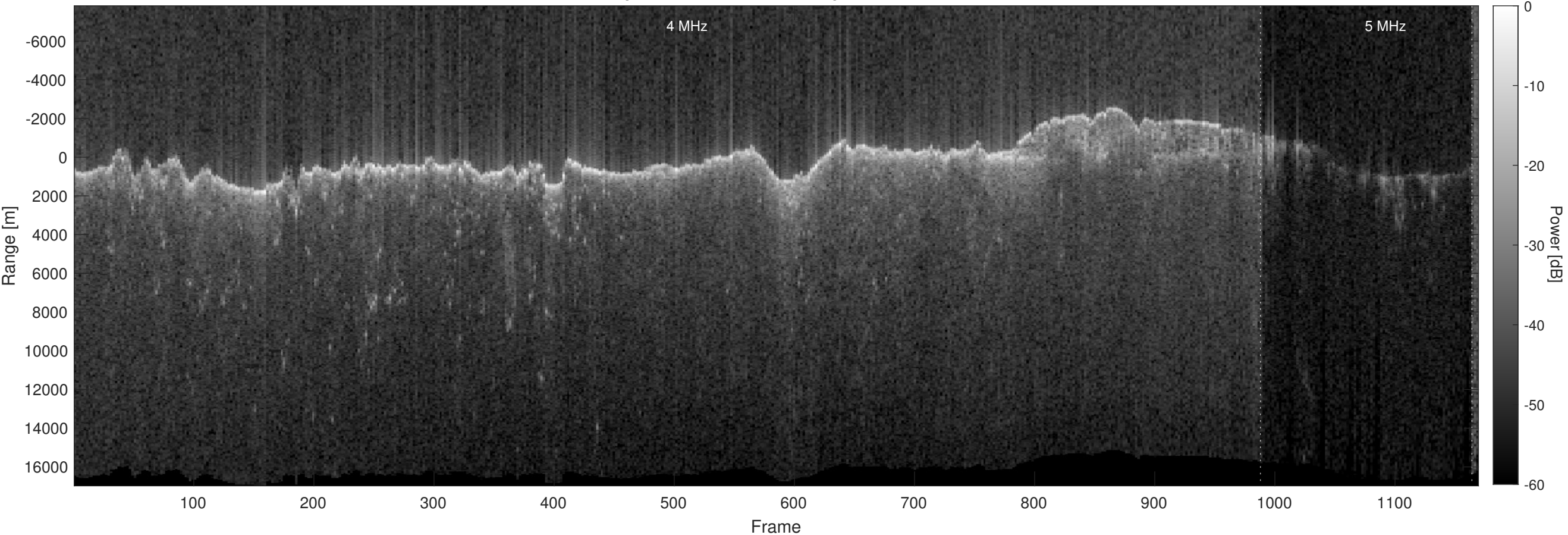
Orbit 10973, Optimized, No Window, Depth-Corrected, Channel 2
