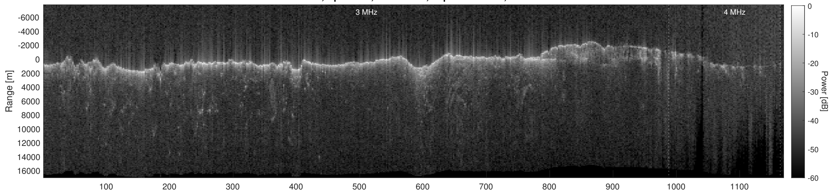
Orbit 10973, Depth-Corrected Cluttergram
