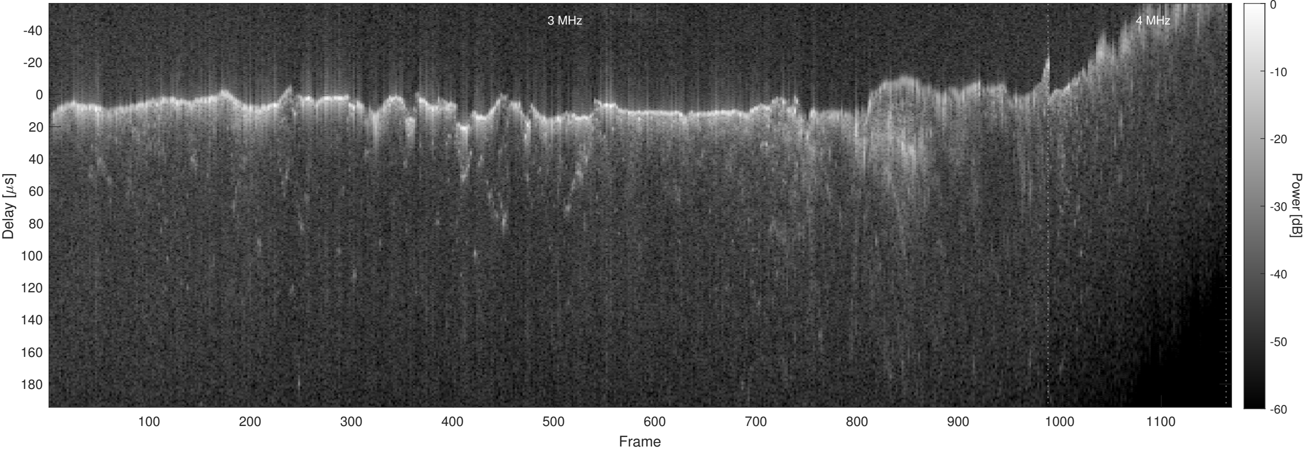
Orbit 10974, Chapman, No Window, Channel 2
