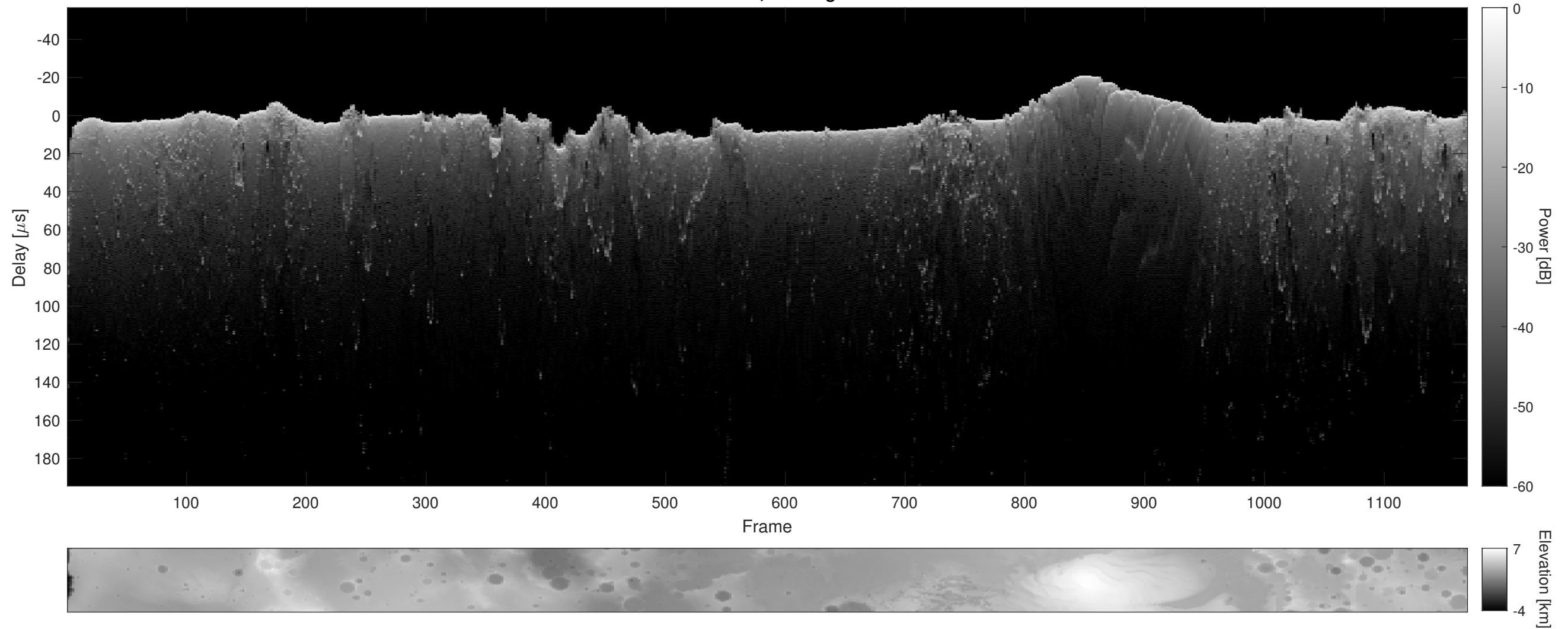
Orbit 10974, Cluttergram
