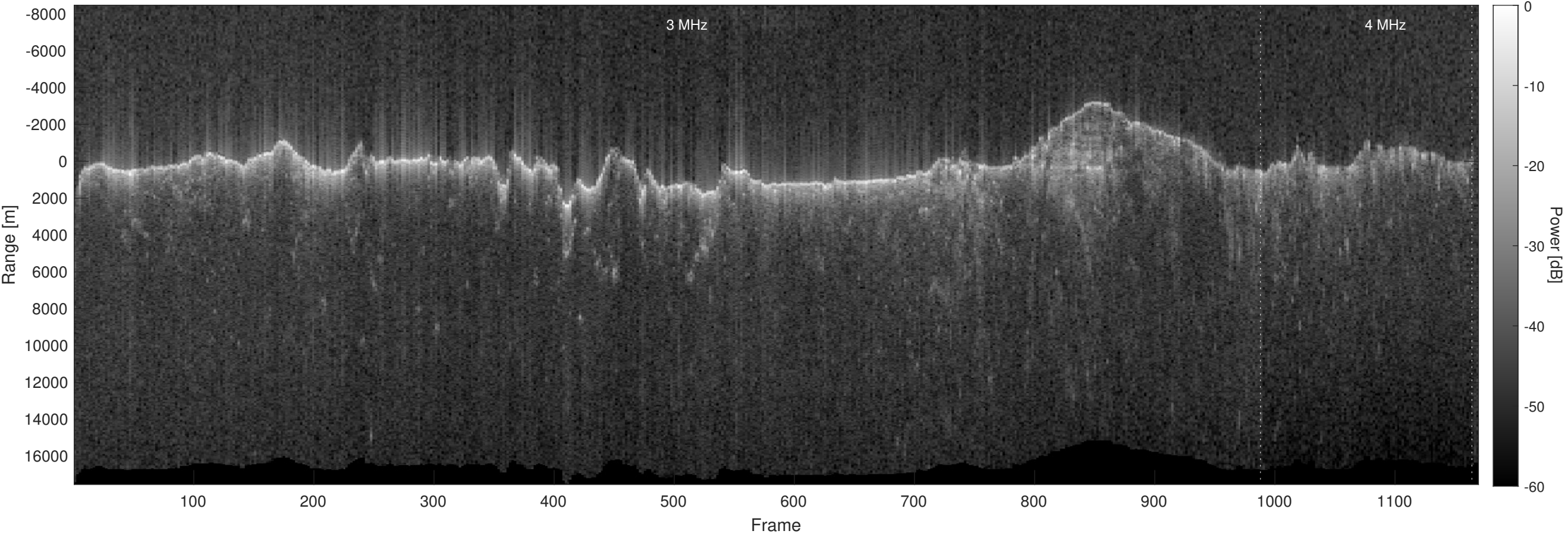
Orbit 10974, Optimized, No Window, Depth-Corrected, Channel 2
