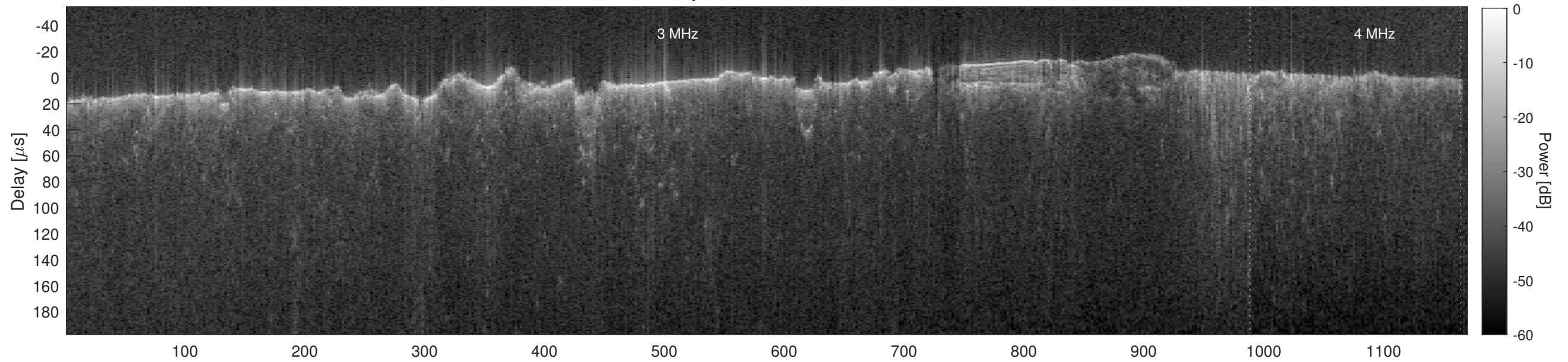
Orbit 10975, Cluttergram
