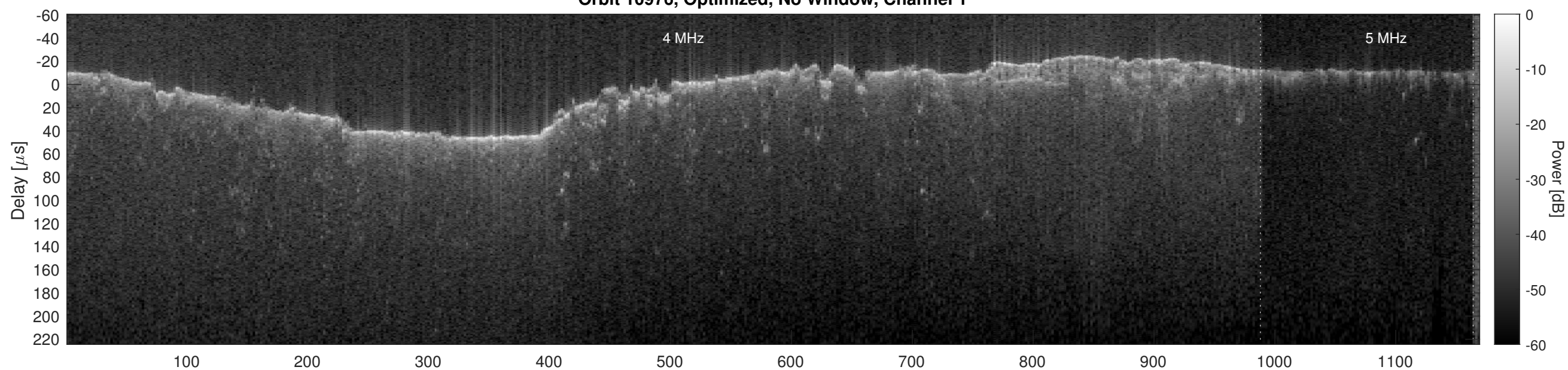
Orbit 10976, Optimized, No Window, Channel 2
