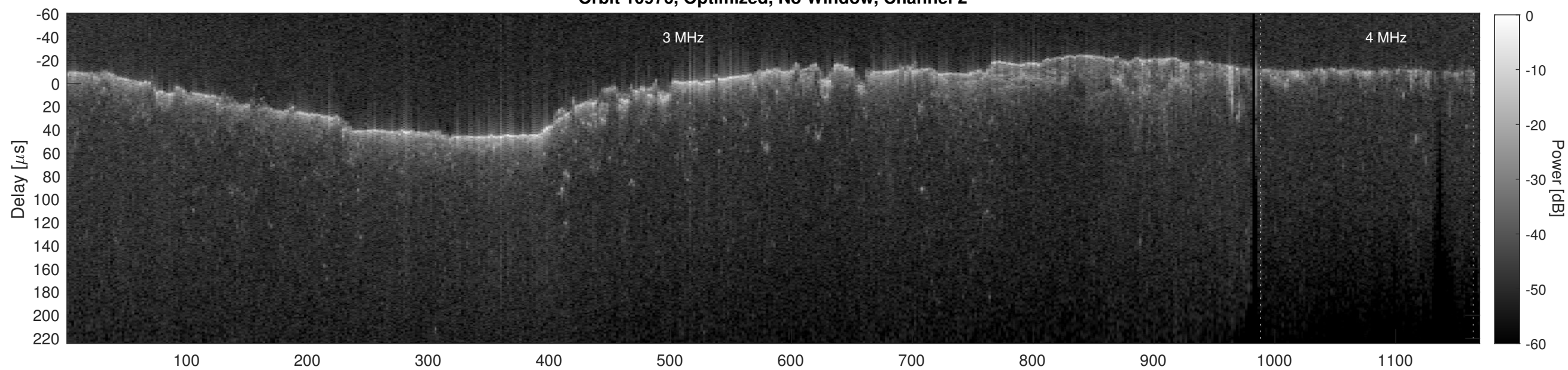
Orbit 10976, Cluttergram
