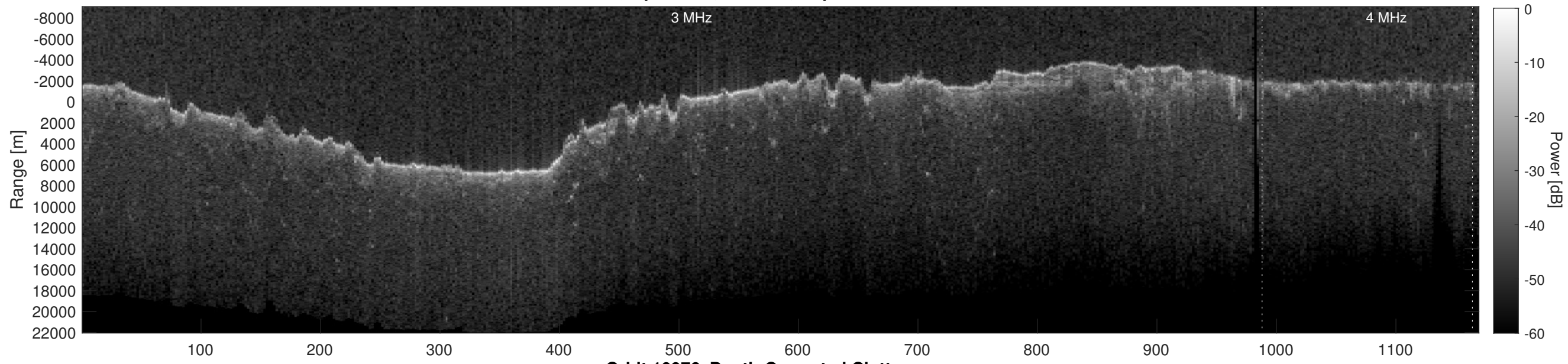
Orbit 10976, Depth-Corrected Cluttergram
