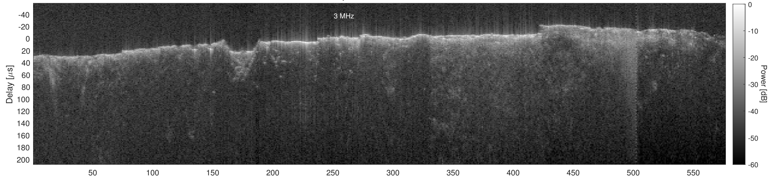
Orbit 10977, Cluttergram
