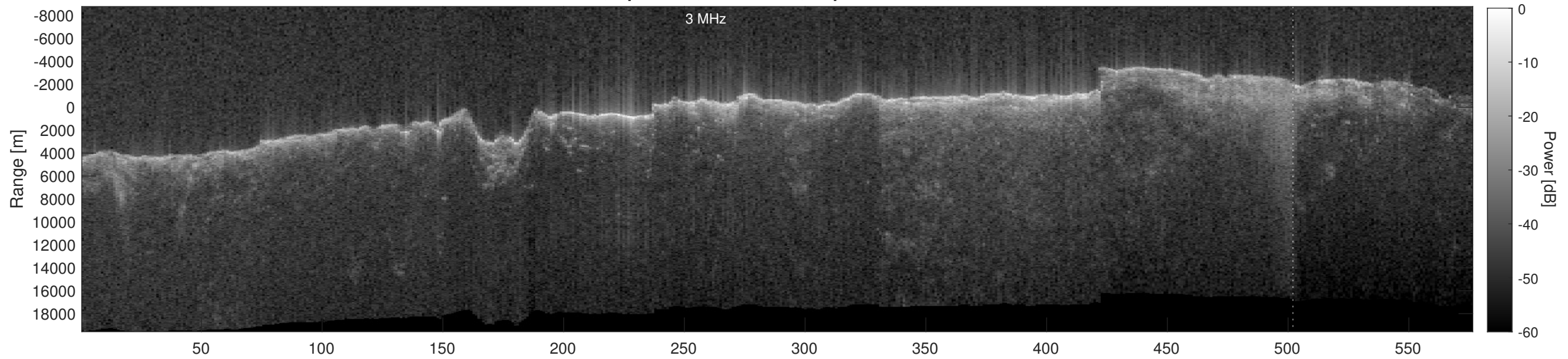
Orbit 10977, Depth-Corrected Cluttergram
