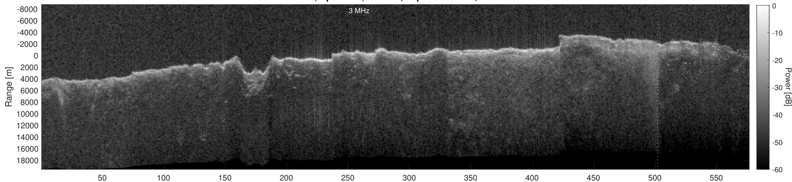
Orbit 10977, Depth-Corrected Cluttergram
