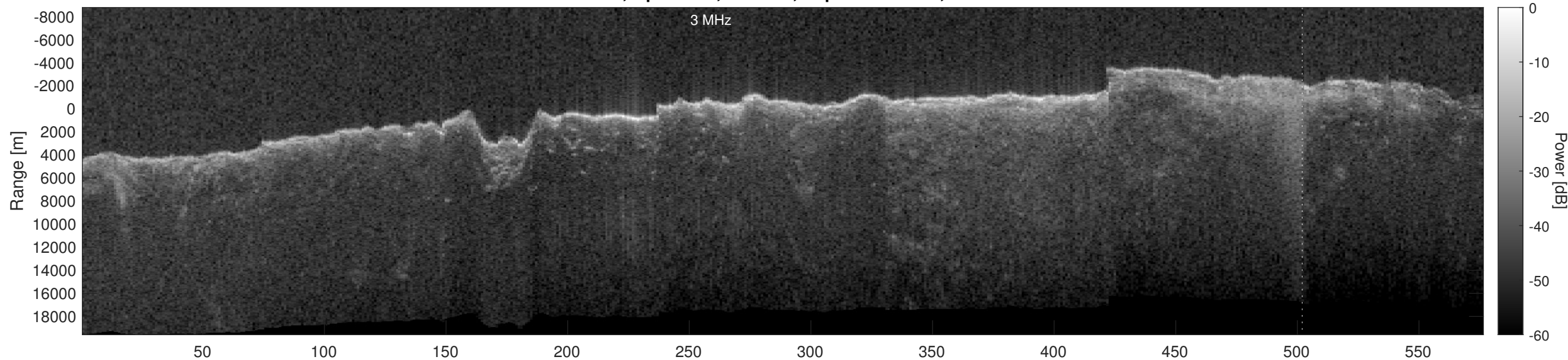
Orbit 10977, Optimized, Window, Depth-Corrected, Channel 2
