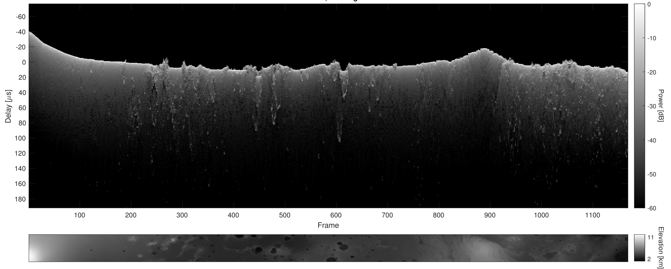
Orbit 10978, Cluttergram
