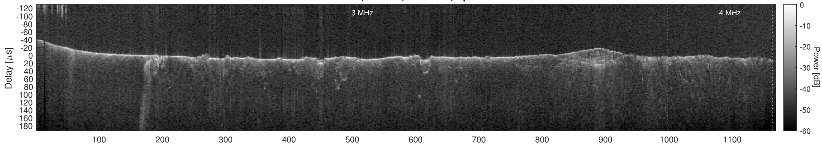
Orbit 10978, Cluttergram
