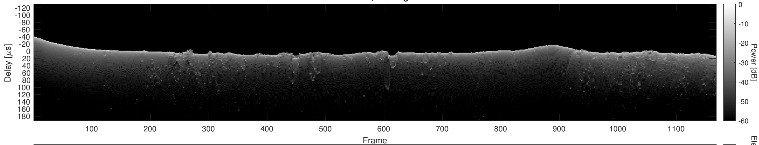
Orbit 10978, Cluttergram
