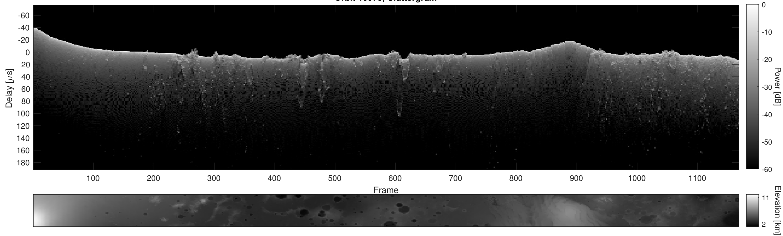
Orbit 10978, Cluttergram
