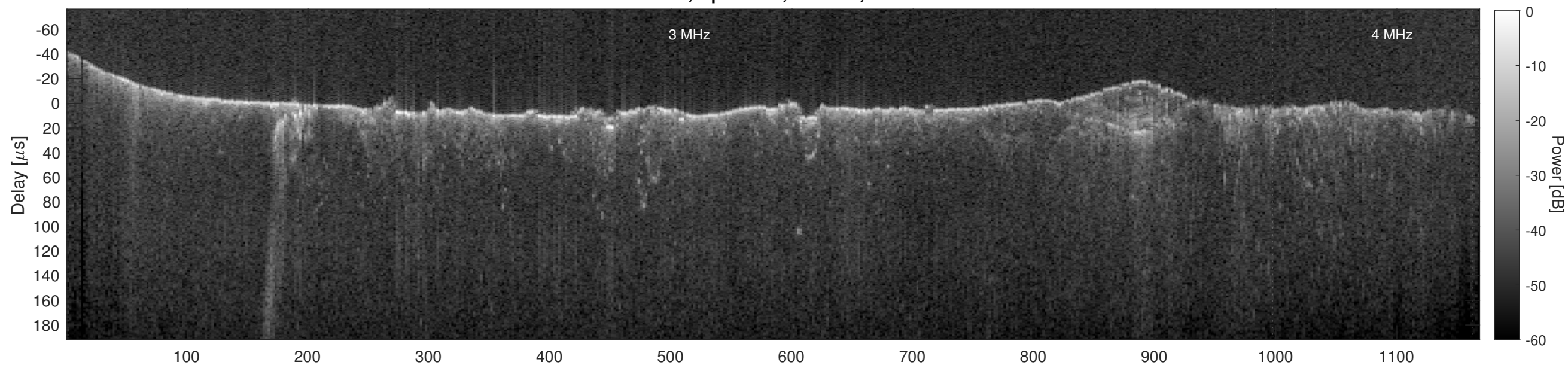
Orbit 10978, Cluttergram
