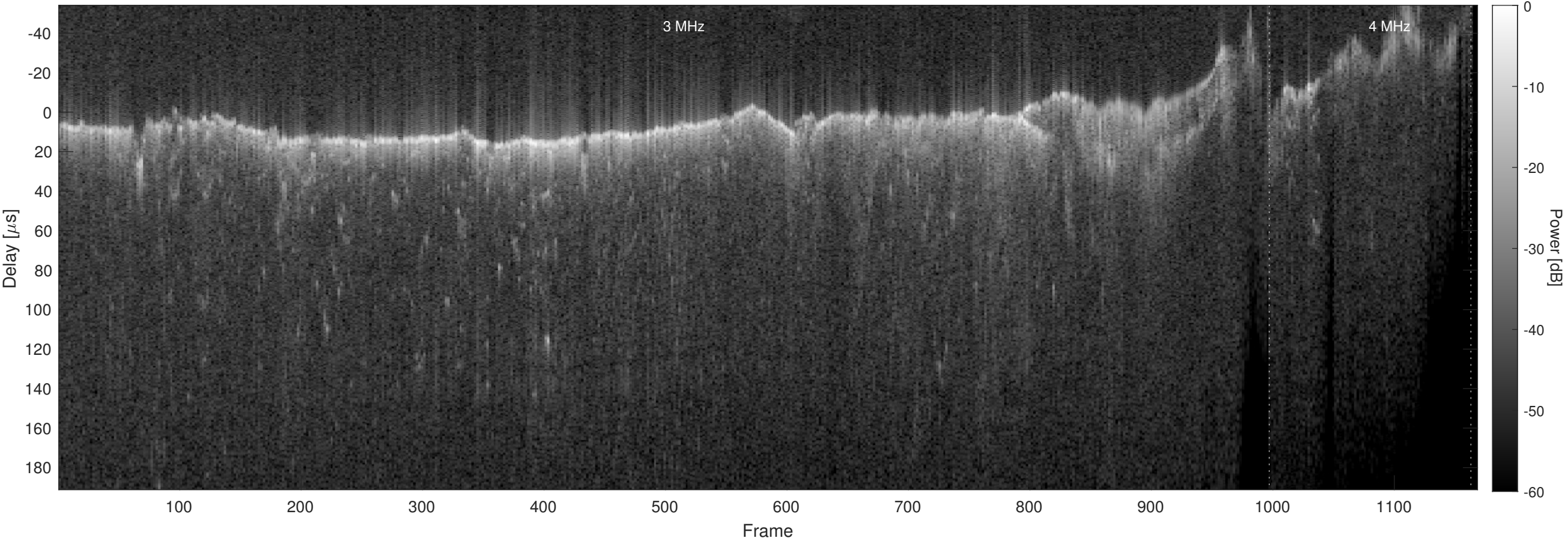
Orbit 10980, Chapman, No Window, Channel 2
