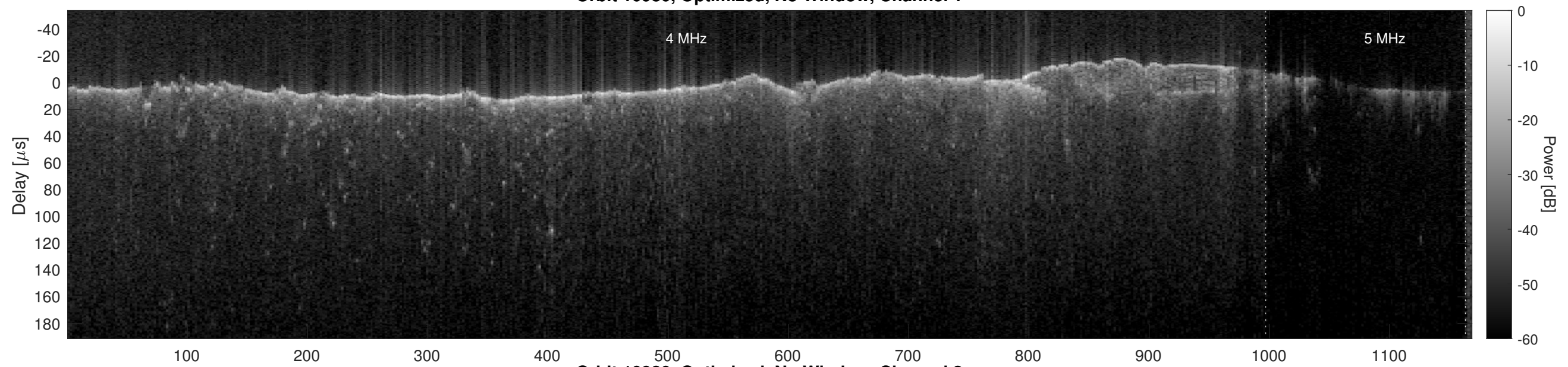
Orbit 10980, Optimized, No Window, Channel 2
