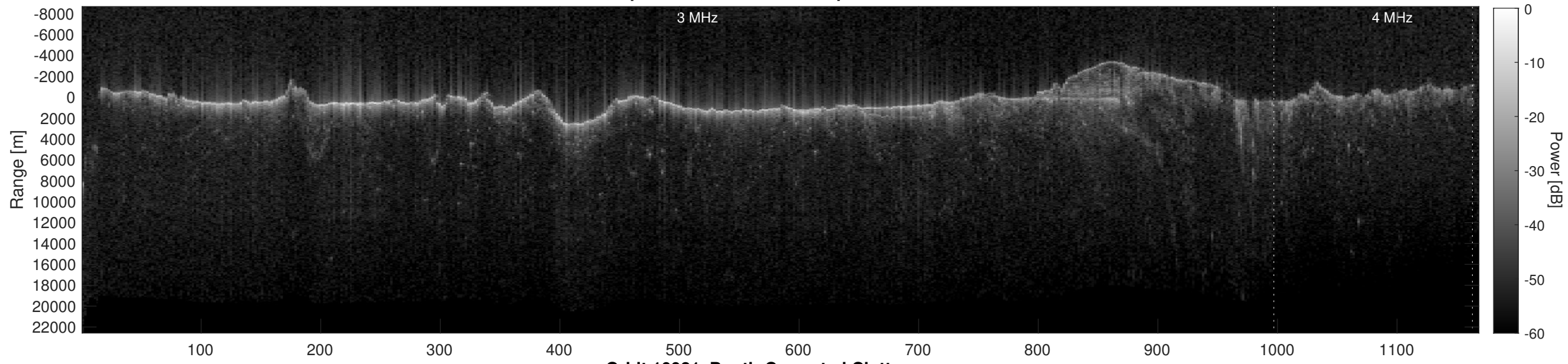
Orbit 10981, Depth-Corrected Cluttergram
