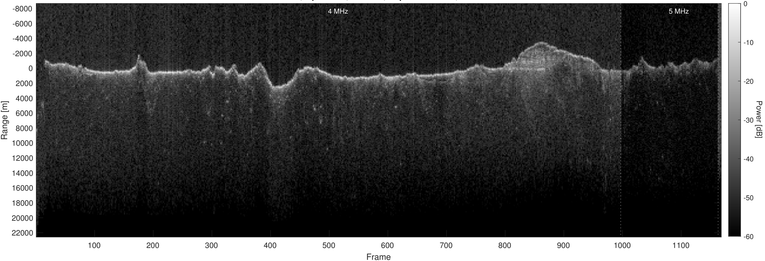
Orbit 10981, Optimized, Window, Depth-Corrected, Channel 2
