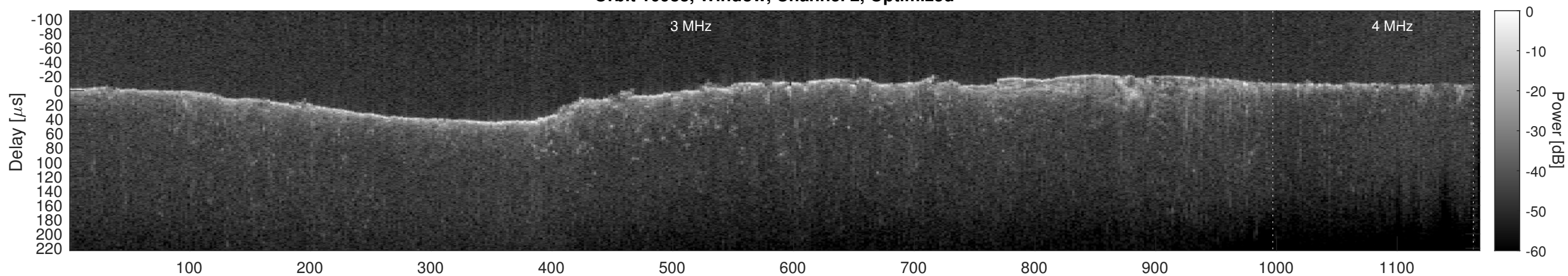
Orbit 10983, Cluttergram
