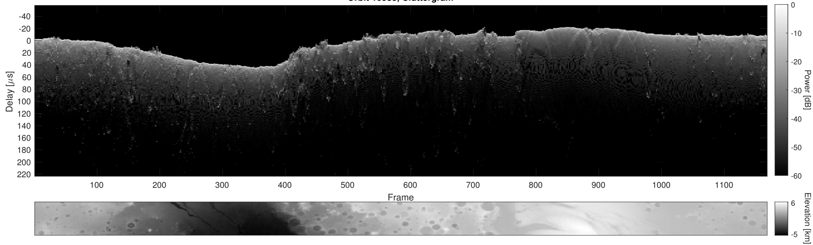
Orbit 10983, Cluttergram
