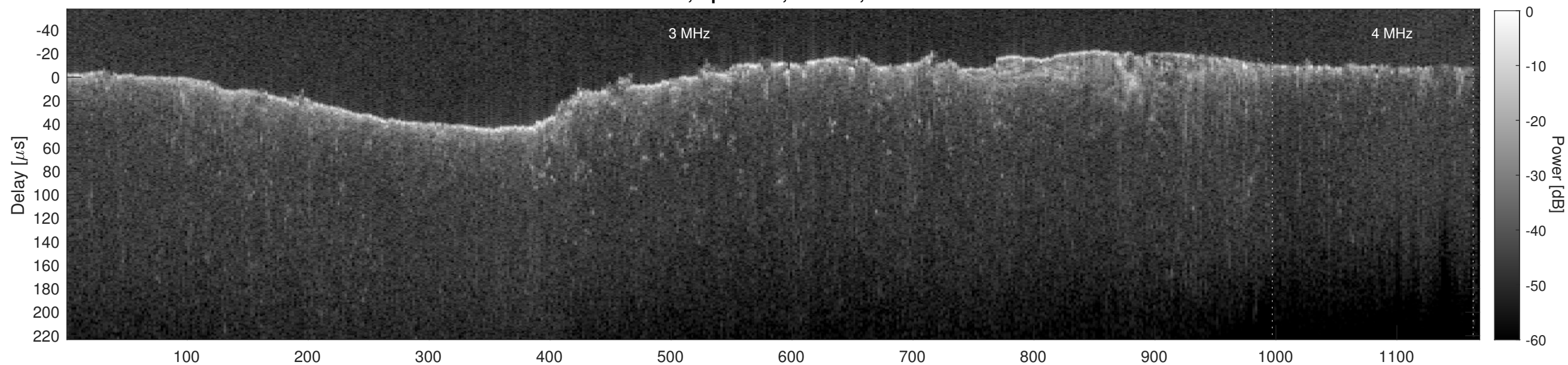
Orbit 10983, Cluttergram
