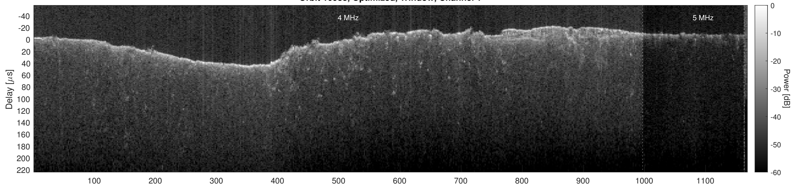
Orbit 10983, Optimized, Window, Channel 2
