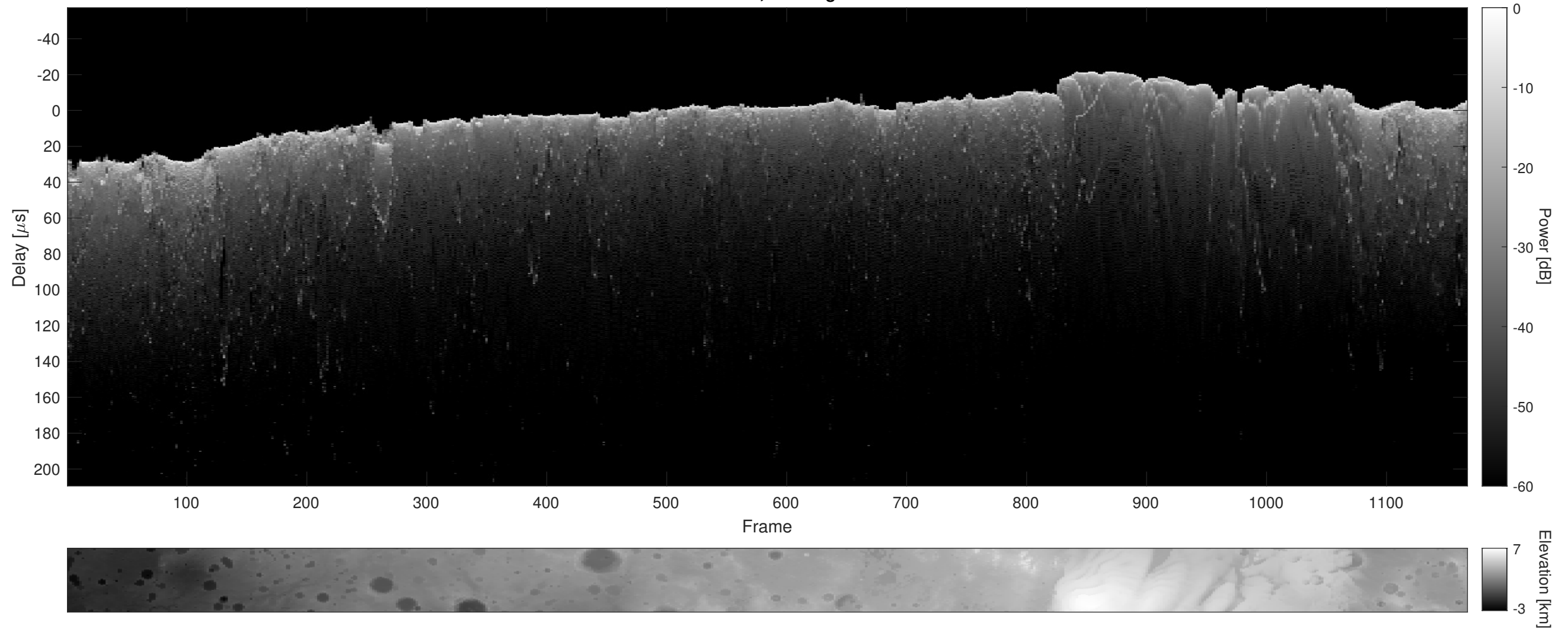
Orbit 10984, Cluttergram
