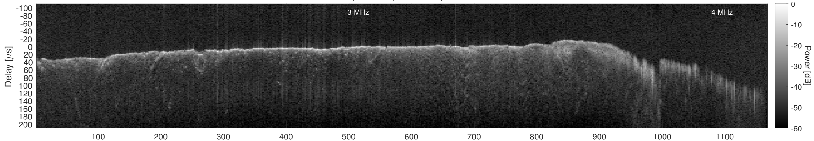
Orbit 10984, Window, Channel 2, Chapman
