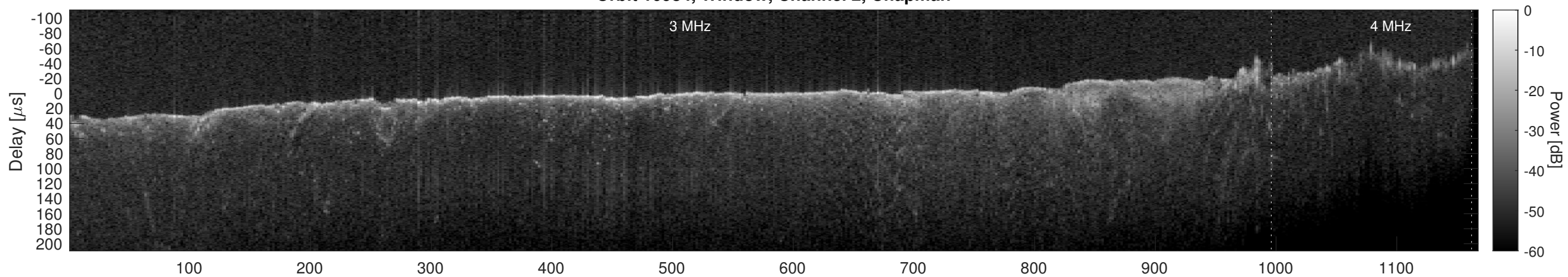
Orbit 10984, Window, Channel 2, Optimized
