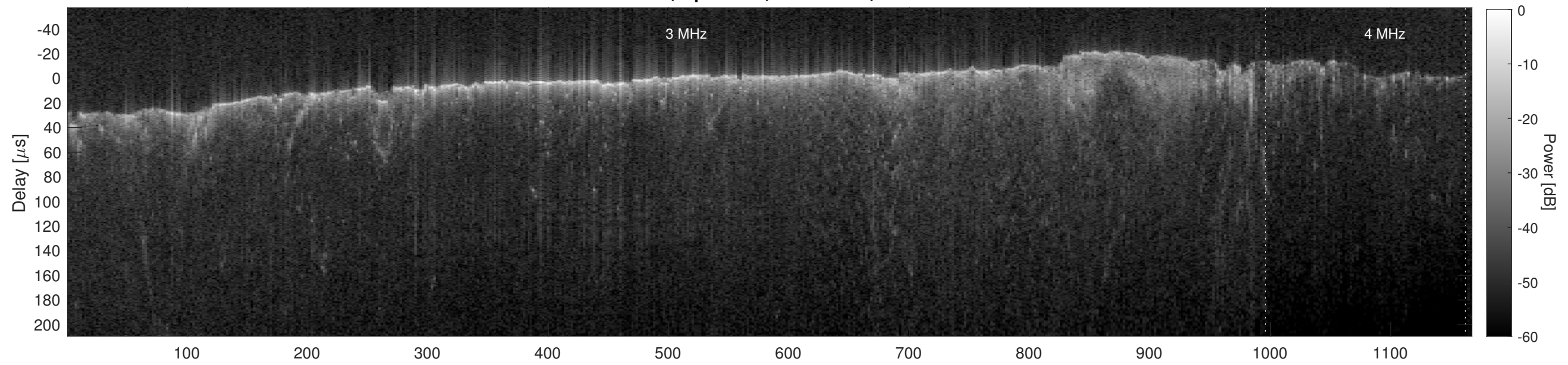
Orbit 10984, Cluttergram
