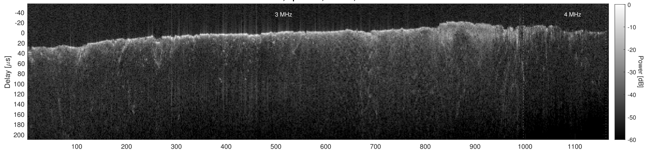
Orbit 10984, Cluttergram
