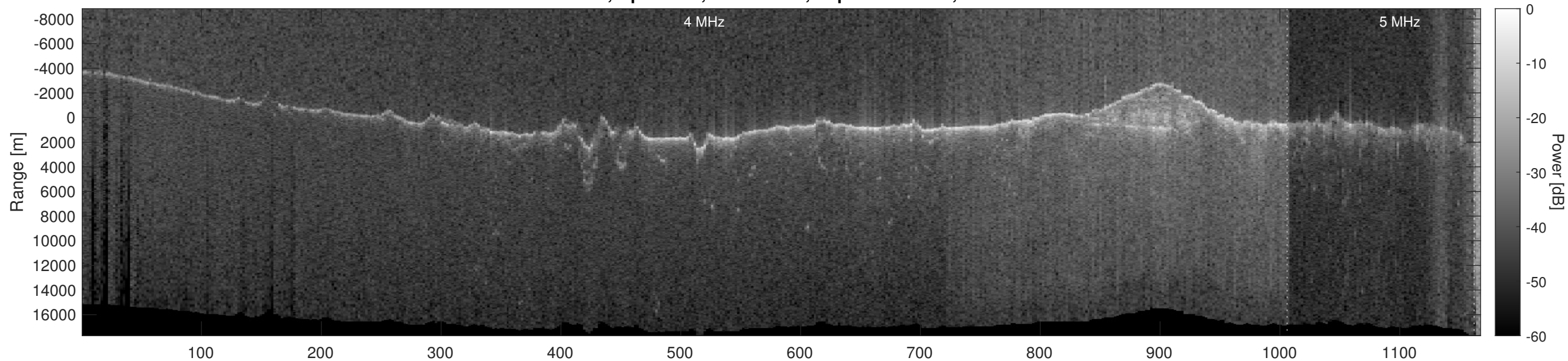
Orbit 10985, Optimized, No Window, Depth-Corrected, Channel 2
