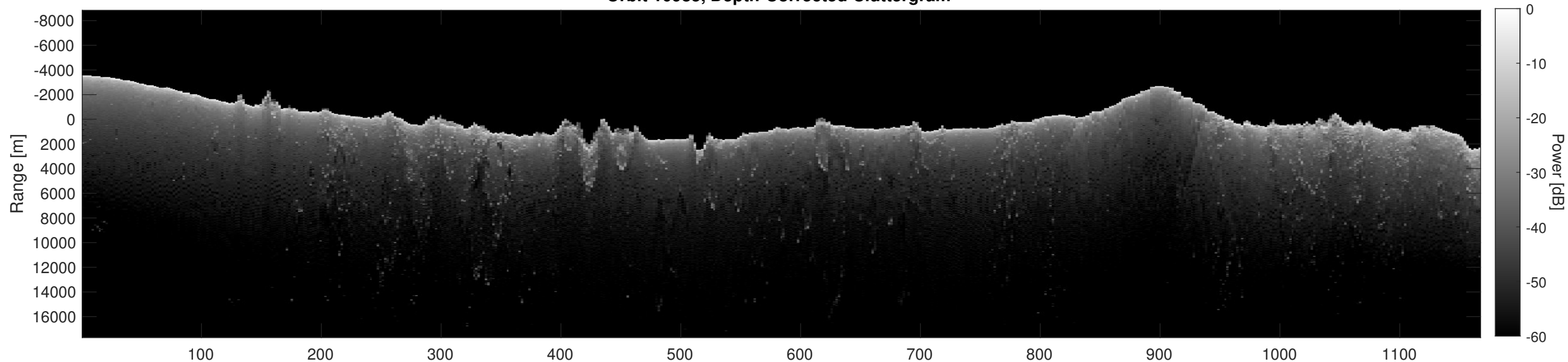
Orbit 10985, Depth-Corrected Cluttergram
