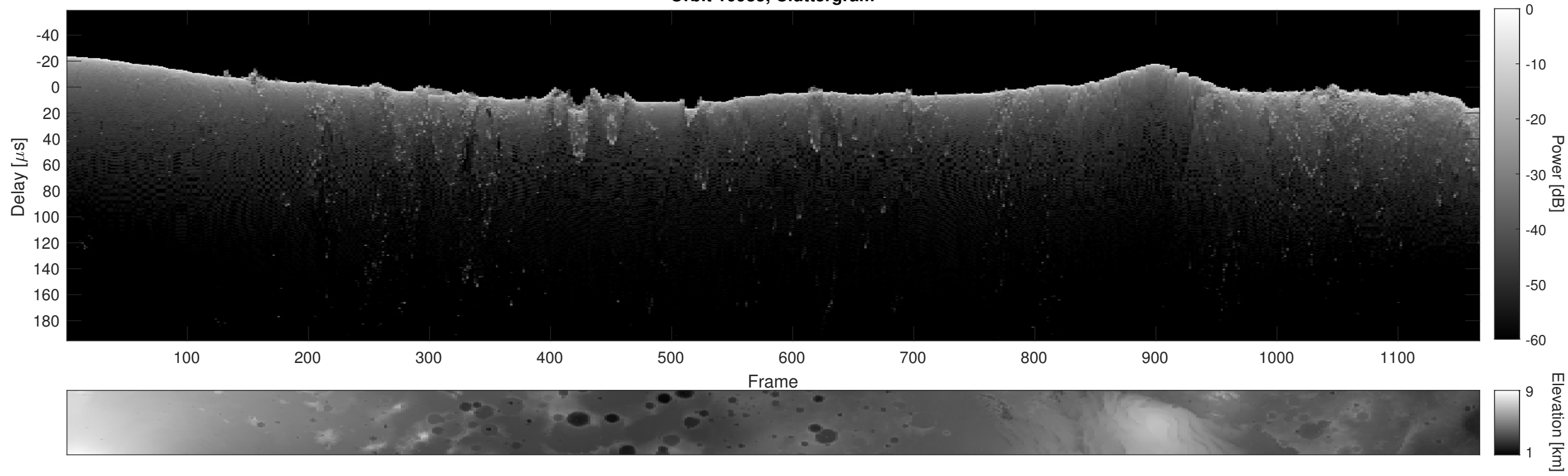
Orbit 10985, Cluttergram
