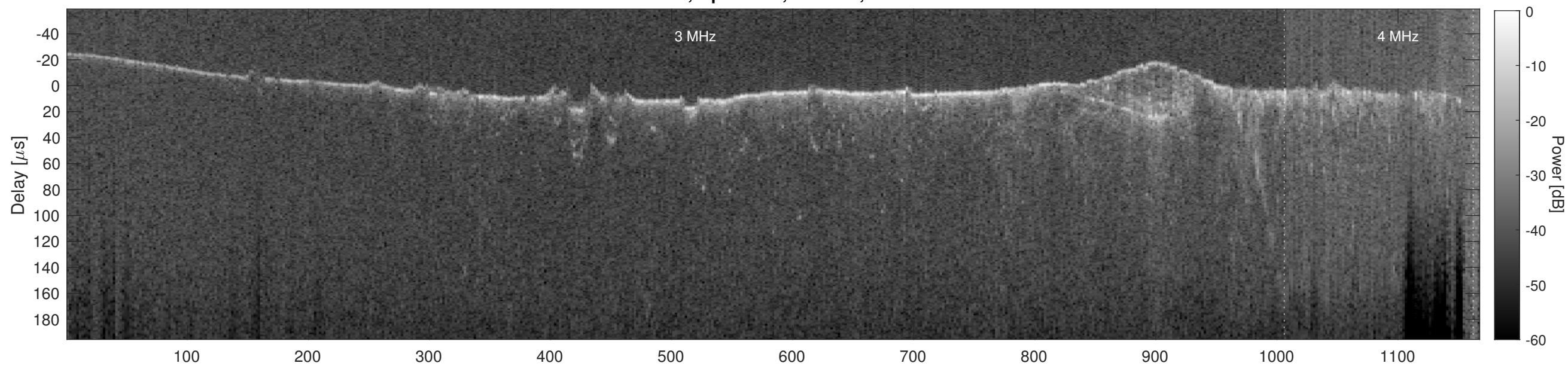
Orbit 10985, Cluttergram
