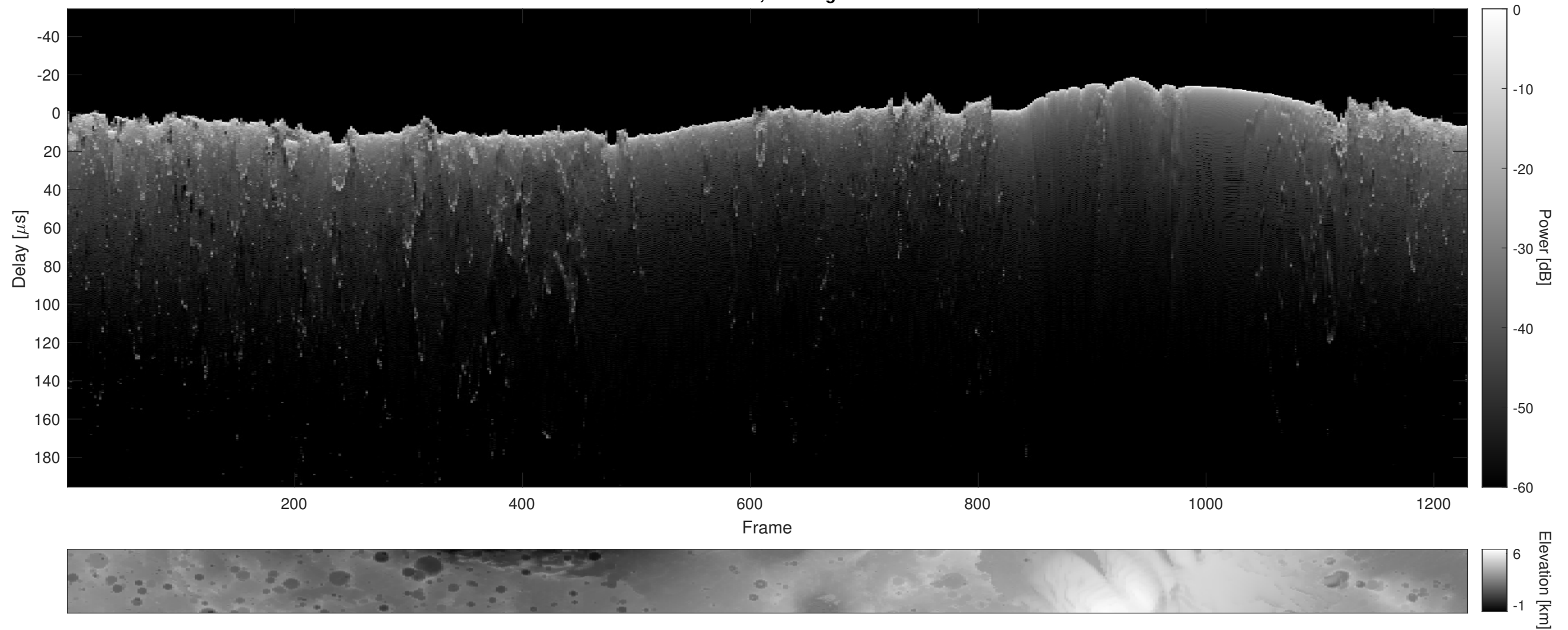
Orbit 10987, Cluttergram
