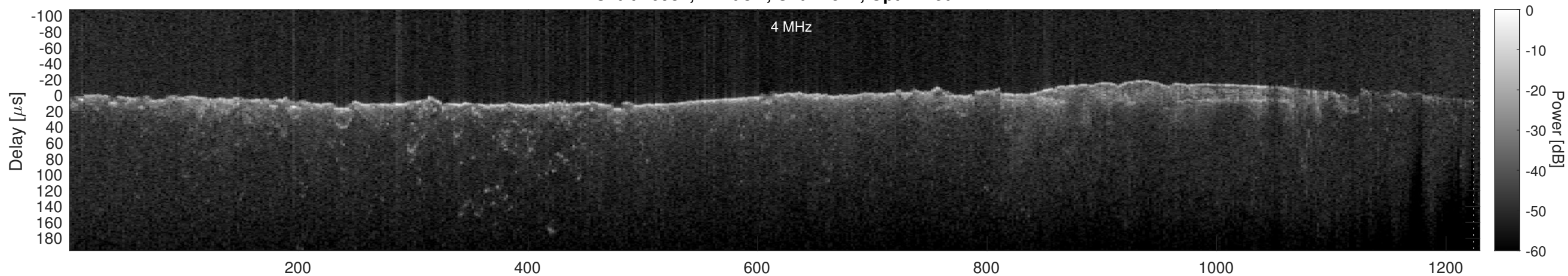
Orbit 10987, Cluttergram
