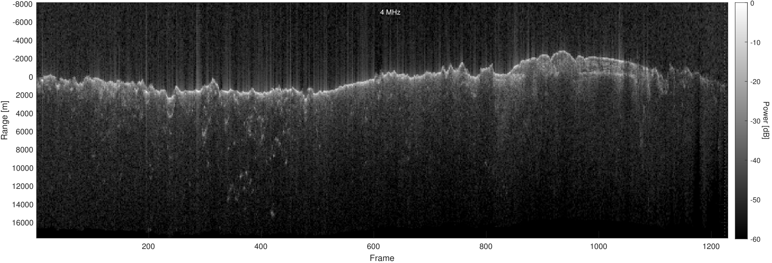
Orbit 10987, Optimized, No Window, Depth-Corrected, Channel 2
