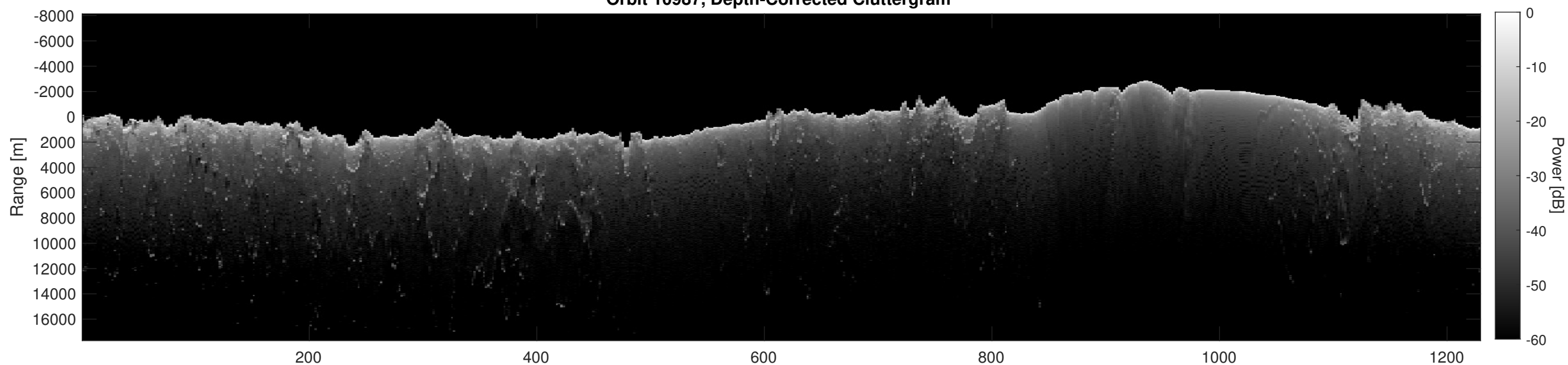
Orbit 10987, Depth-Corrected Cluttergram
