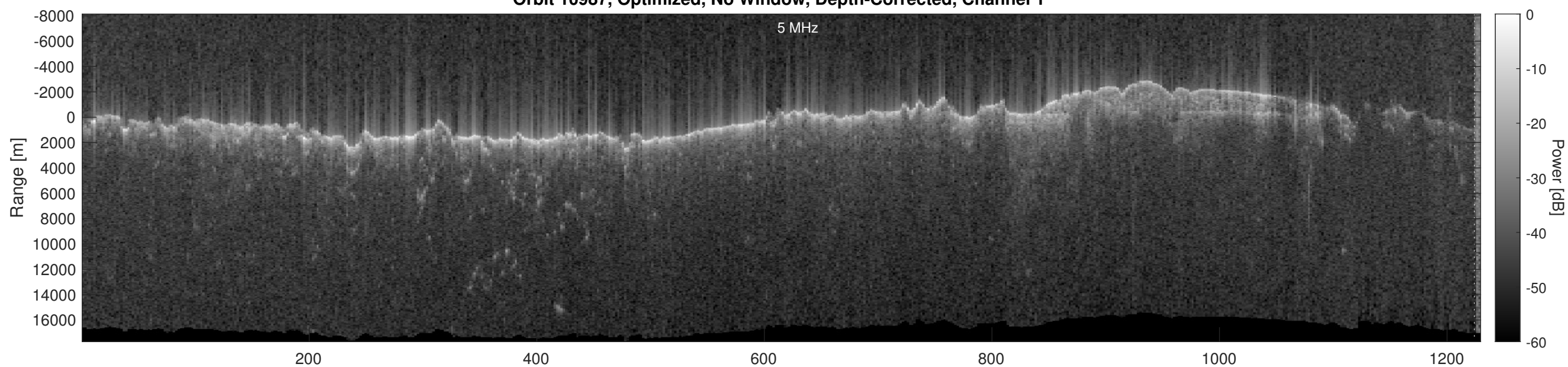
Orbit 10987, Optimized, No Window, Depth-Corrected, Channel 2
