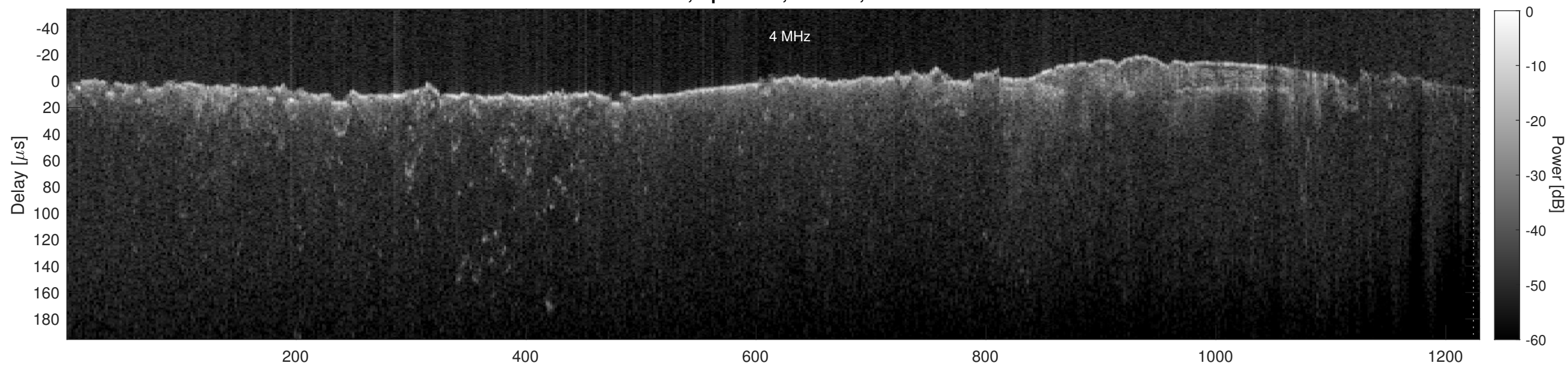
Orbit 10987, Cluttergram
