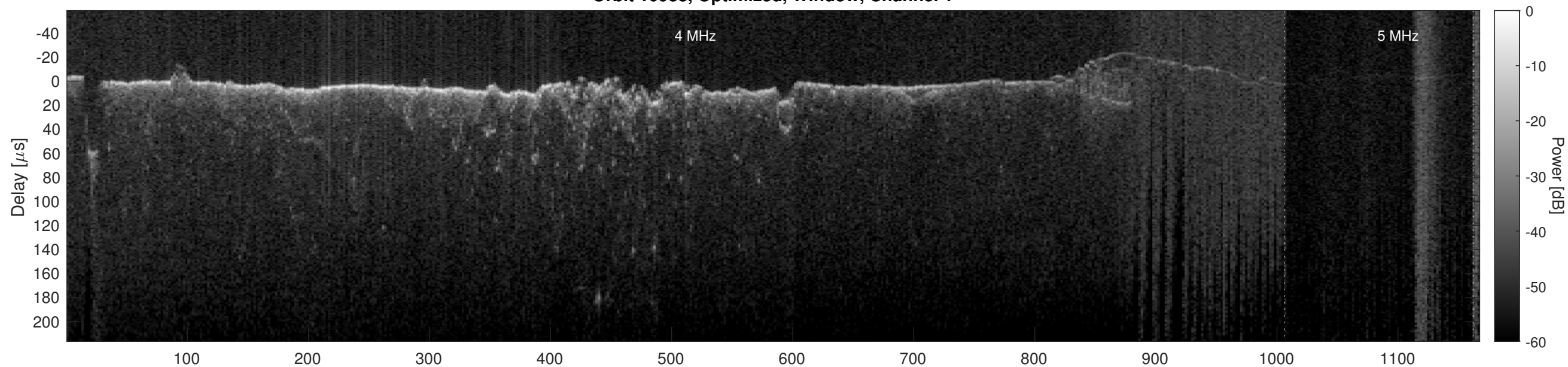
Orbit 10988, Optimized, Window, Channel 2
