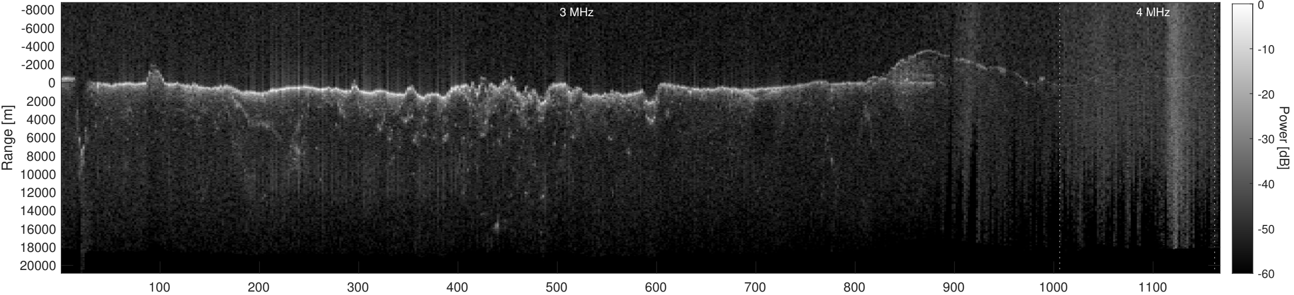
Orbit 10988, Depth-Corrected Cluttergram
