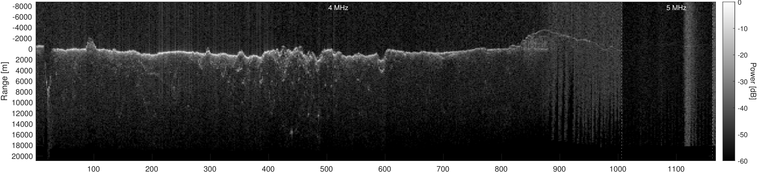
Orbit 10988, Optimized, Window, Depth-Corrected, Channel 2
