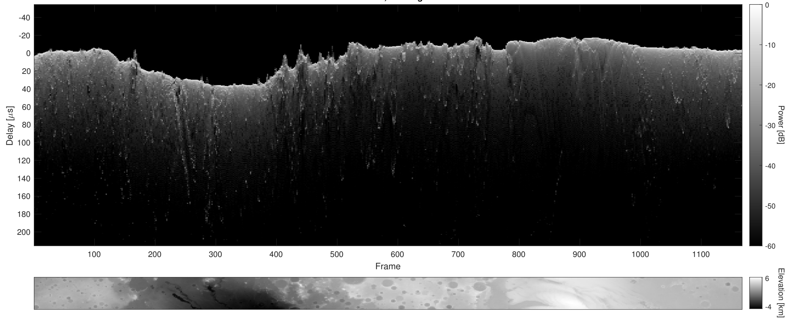
Orbit 10990, Cluttergram
