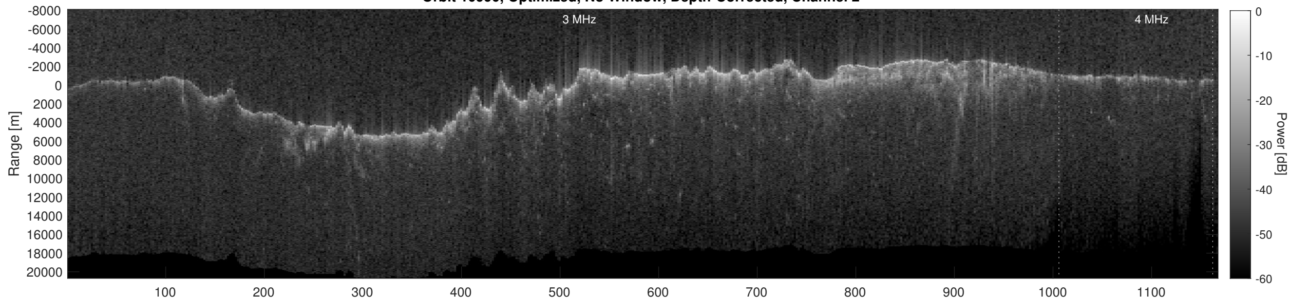
Orbit 10990, Depth-Corrected Cluttergram
