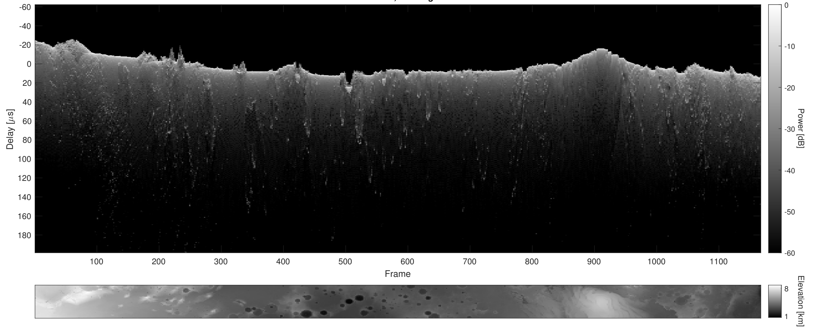
Orbit 10992, Cluttergram
