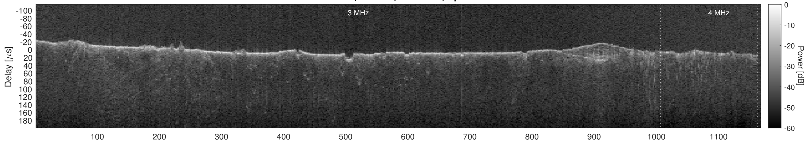
Orbit 10992, Cluttergram
