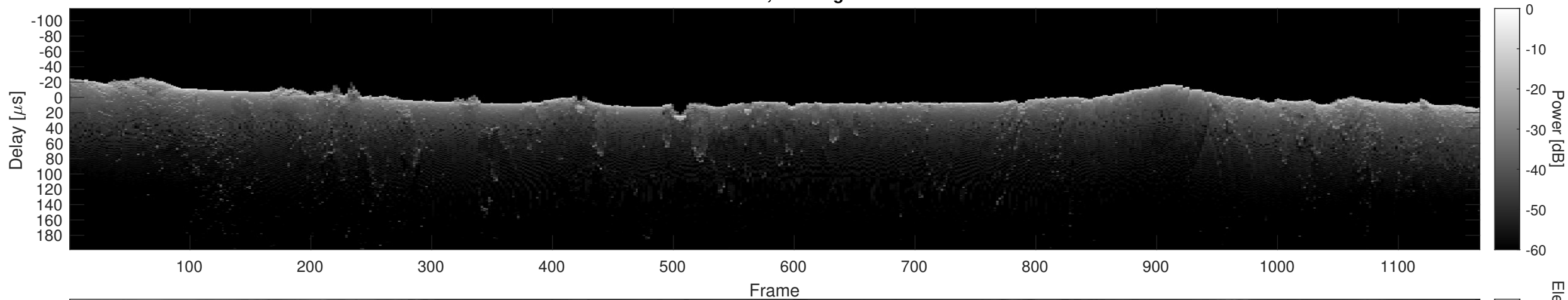
Orbit 10992, Cluttergram
