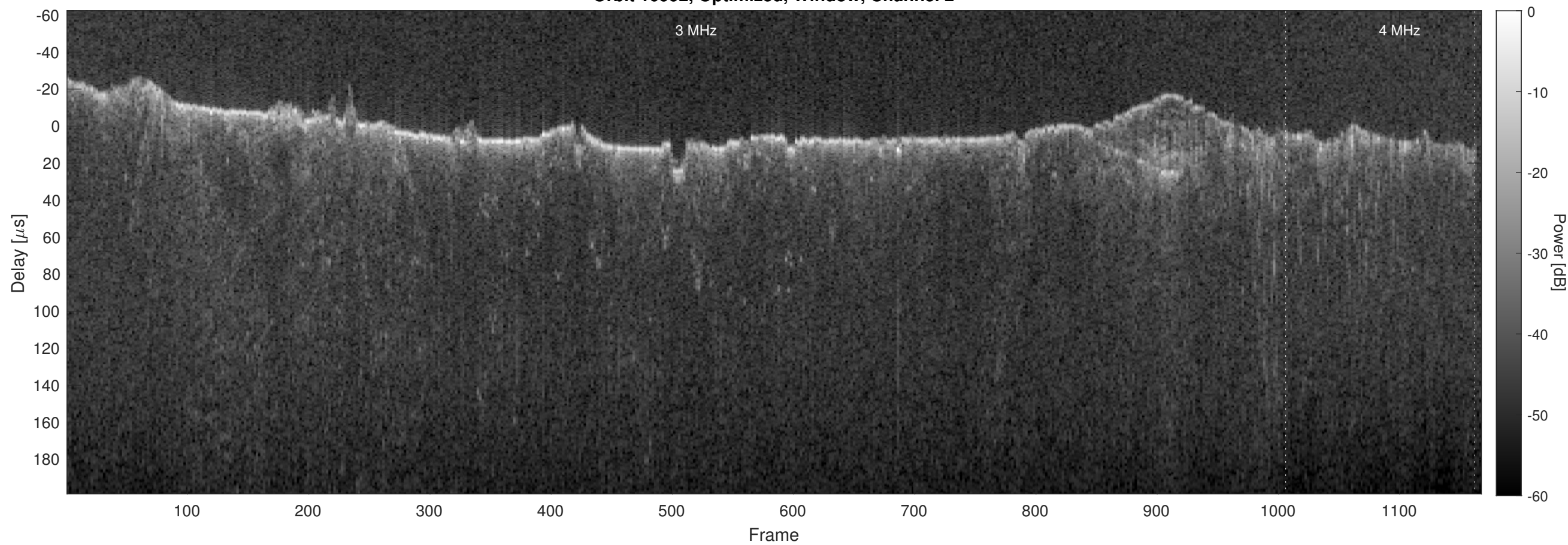
Orbit 10992, Optimized, Window, Channel 2
